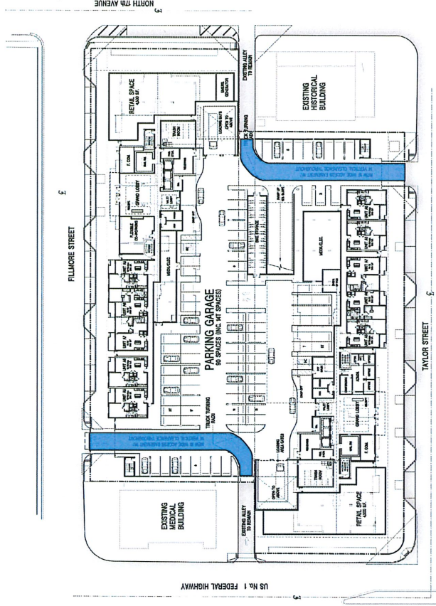
ALLEY ACCESS EASEMENT LEVEL: 1 SCALE: 1/8" = 1'-0"
