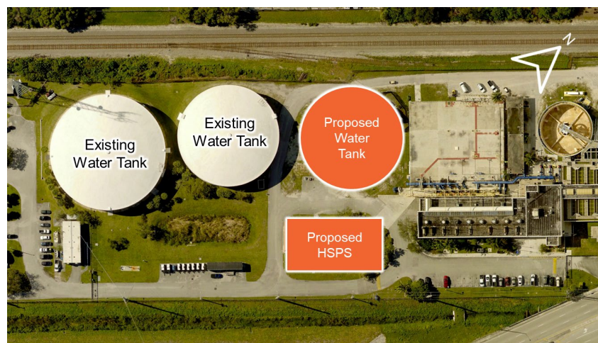
Figure 2-9: Planned Storage and Pumping Improvements
