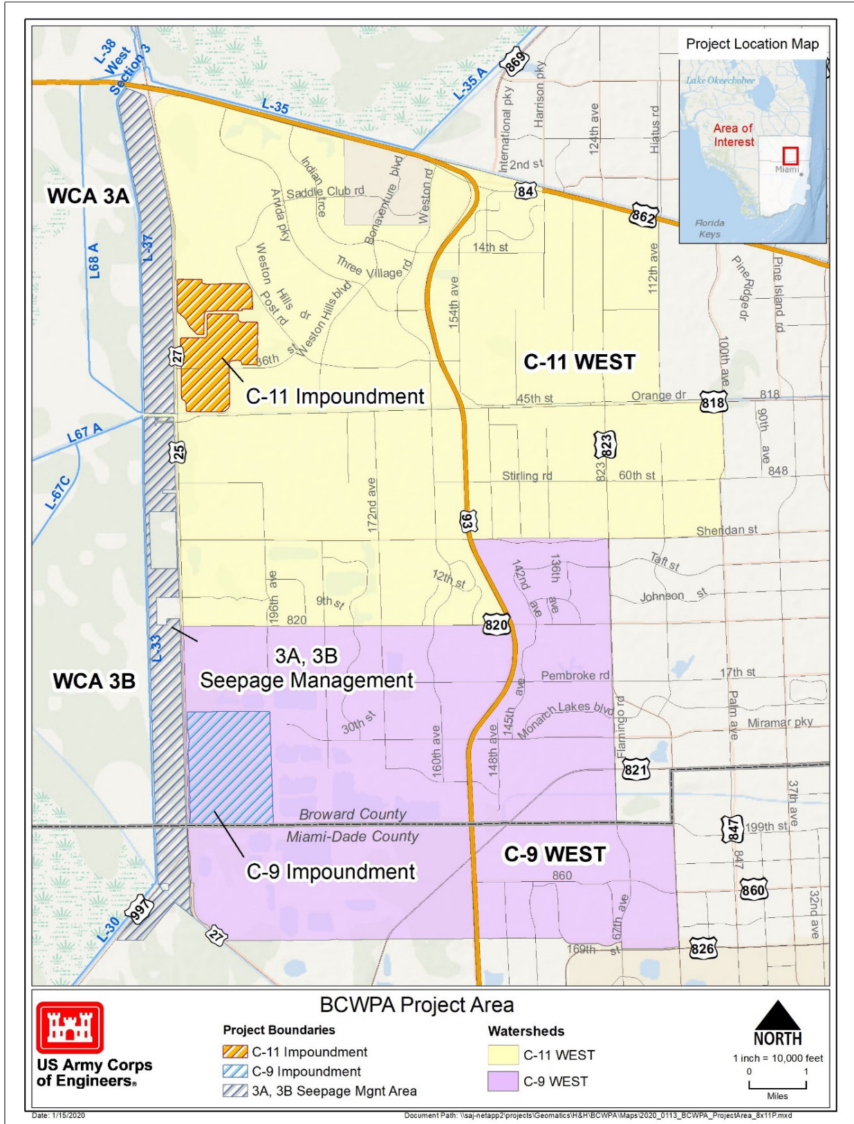
Figure 7-17. Broward County Water Preserve Areas project area and features.
