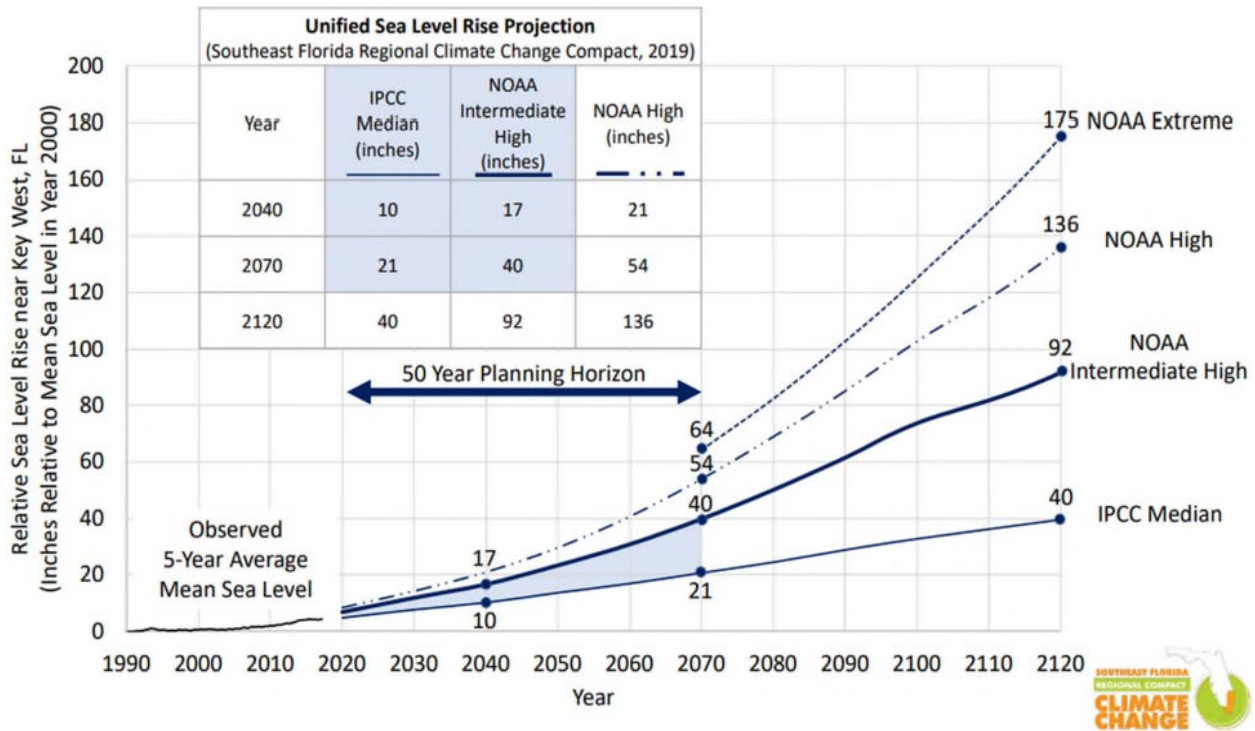
Figure 6.2 Sea Level Rise Projections (2019)
