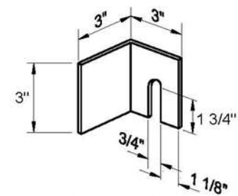
ANGLE DETAIL
