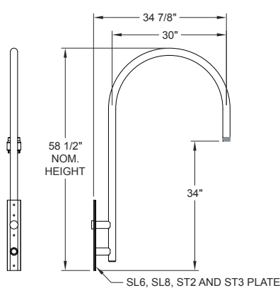
BCR 30IN 1A B0 ((1) 30IN Bolt-on SL6, SL8, ST2 or ST3)
