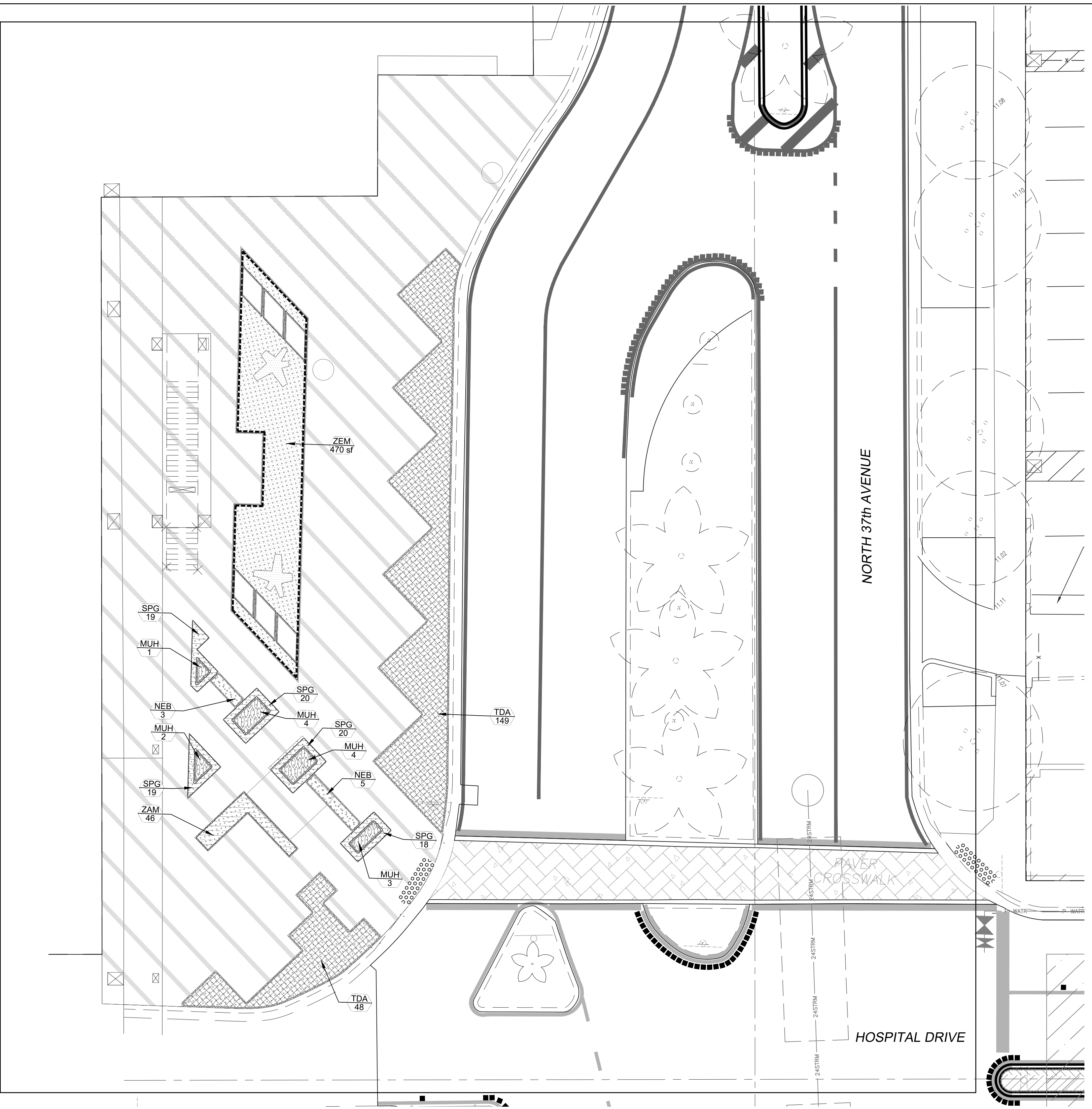
2 ENLARGEMENT PLAN: CORNER PLAZA - UNDERSTORY PLAN
