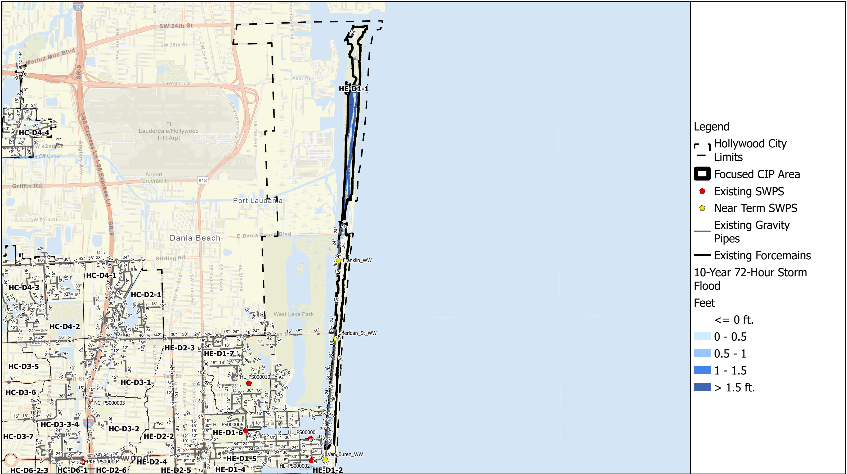
Current Conditions Flooding in CIP Area North Beach and South Central Beach 10-year Design Storm
