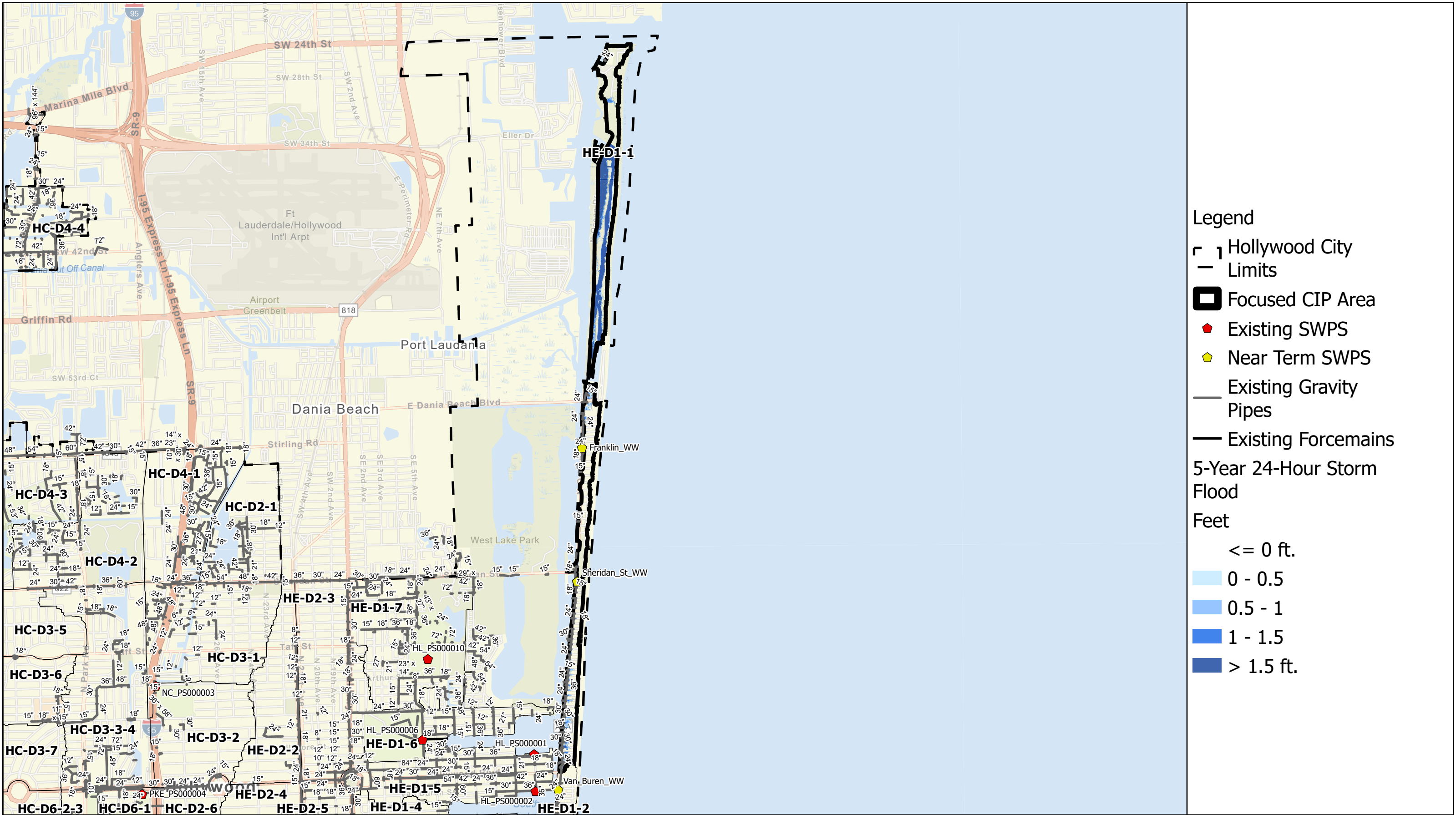
Current Conditions Flooding in CIP Area North Beach and South Central Beach 5-year Design Storm
