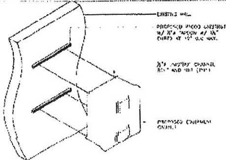
CABINET MOUNTING DETAIL 2
