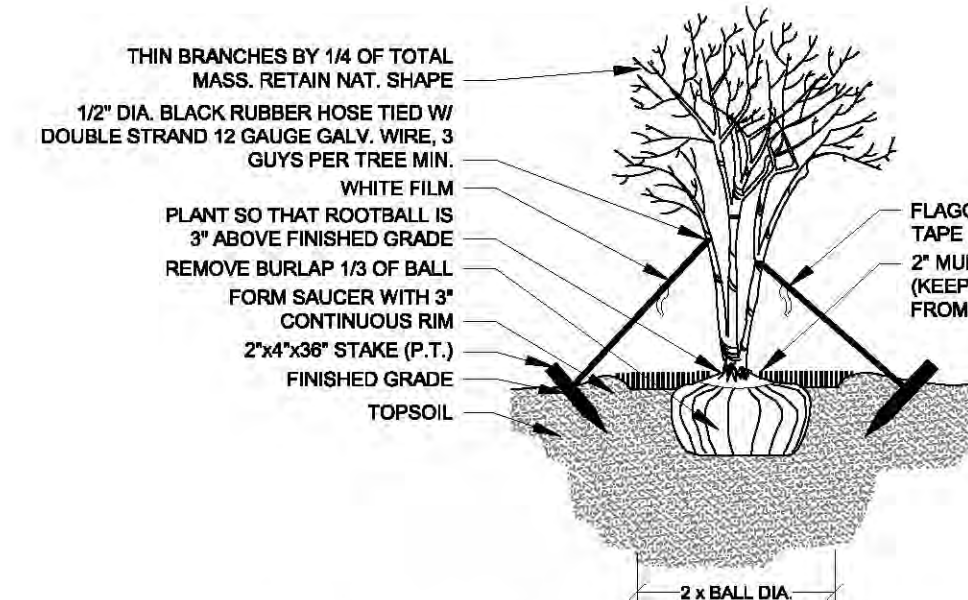
MULTI-TRUNK PLANTING & GUYING NOT TO SCALE
