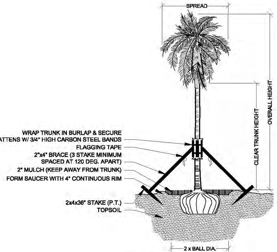
PALM PLANTING - ANGLE STAKE NOT TO SCALE
