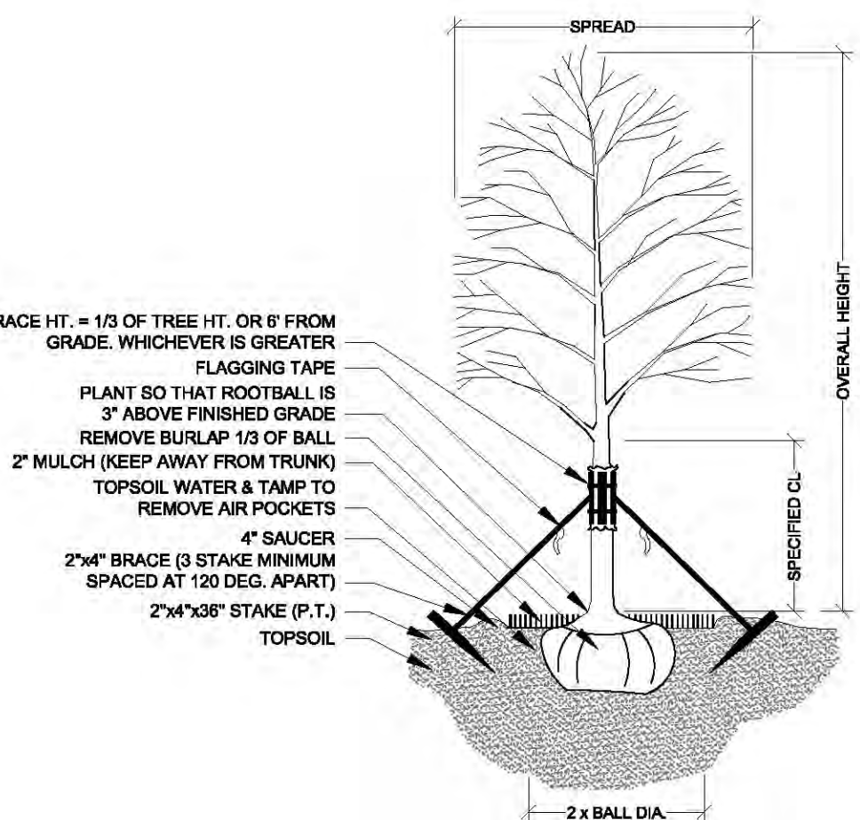
TREE PLANTING & STAKING NOT TO SCALE
