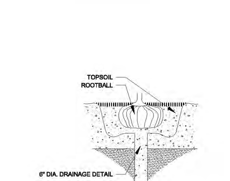
DRAINAGE TESTING DETAIL NOT TO SCALE
