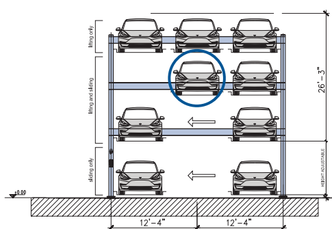
2. Slide-motion initiated.
