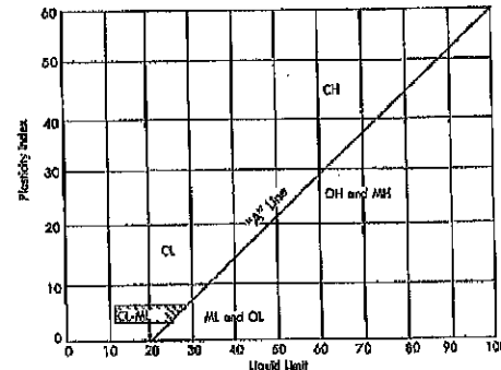
Plasticity Chart
