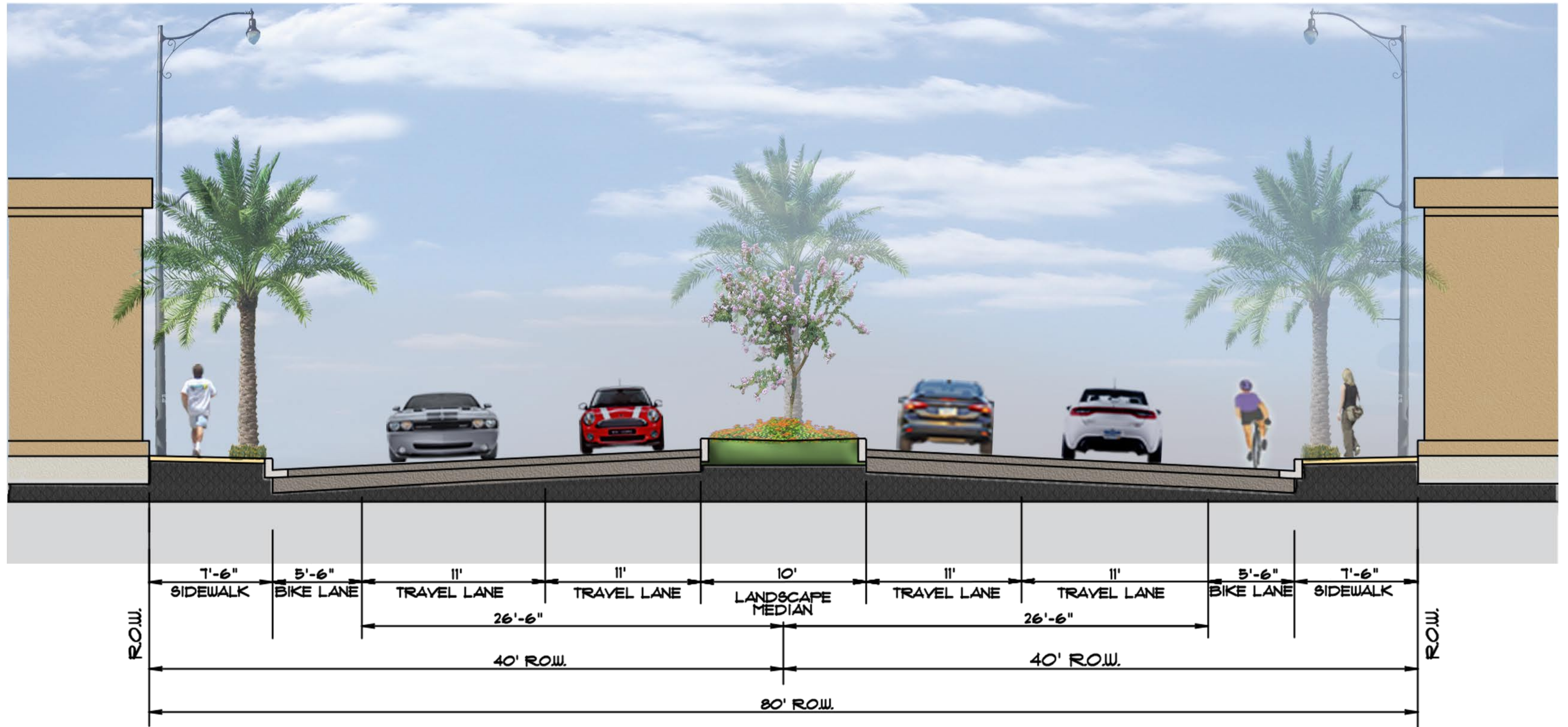
S. Federal Highway Corridor - Proposed Street Section with Median
