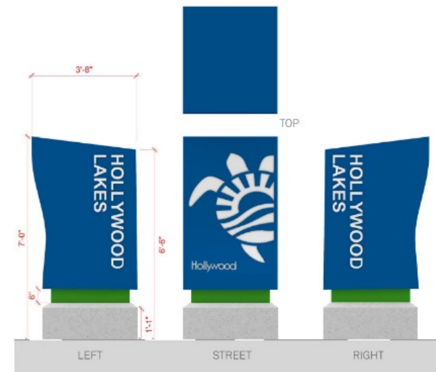
Type E Option 2 – Wave Shape
