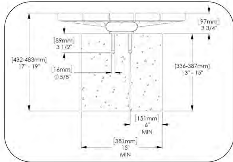
Fig. 2 – anchor hole size
