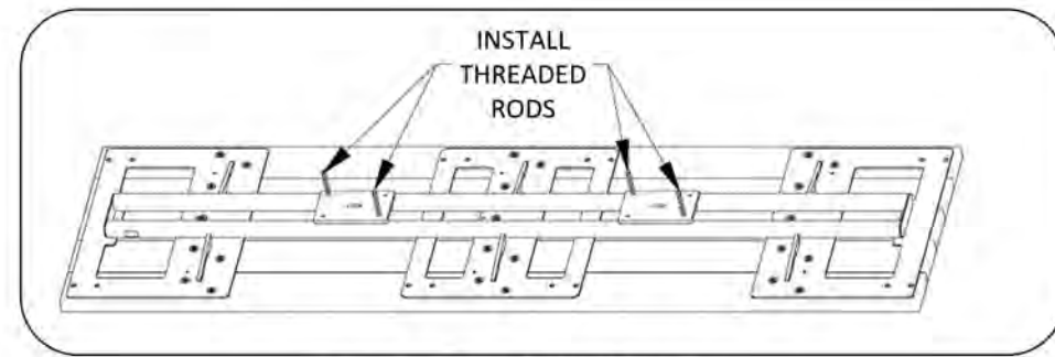
Fig. 1 – Threaded rod locations
