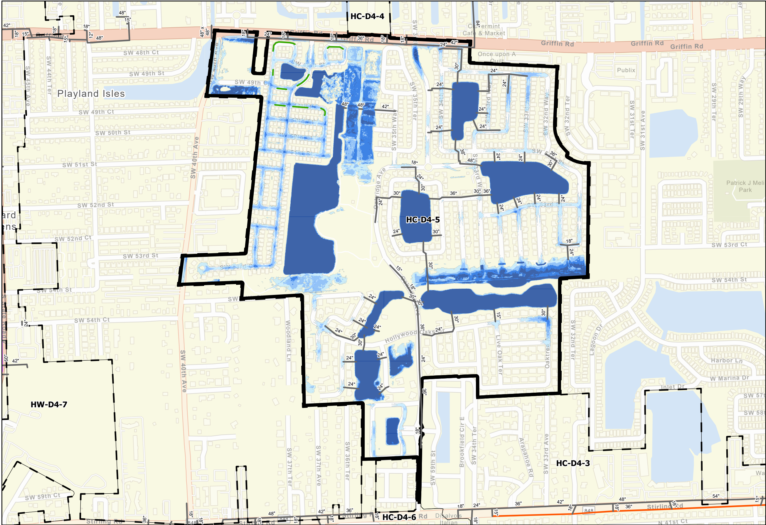
Predicted Flooding Reduction and Proposed ALT 1 CIP for 5-year Design Storm in CIP Area Oakridge / Mapleridge
