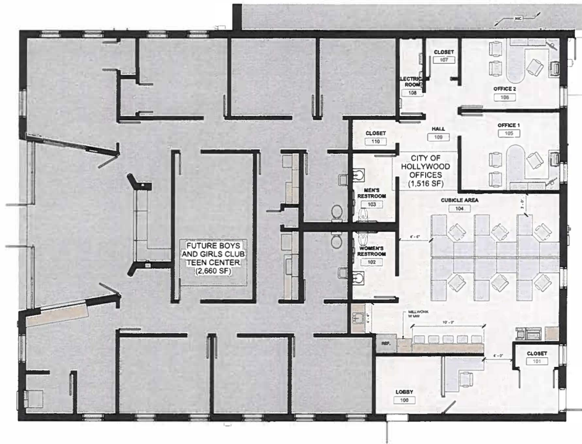
1 FIRST FLOOR PLAN - FFE 144' x 112'
