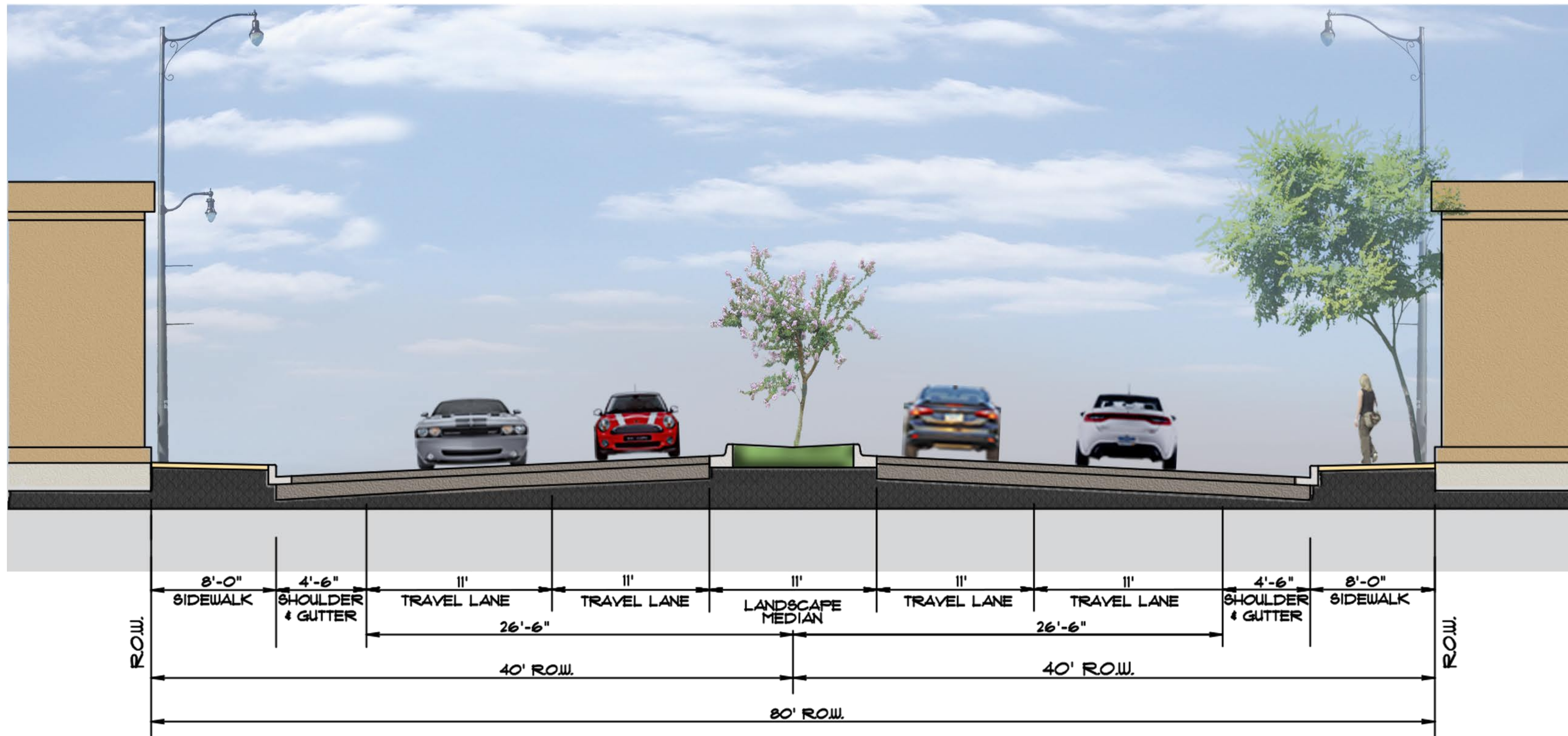
N. Federal Highway Corridor - Existing Street Section with Median
