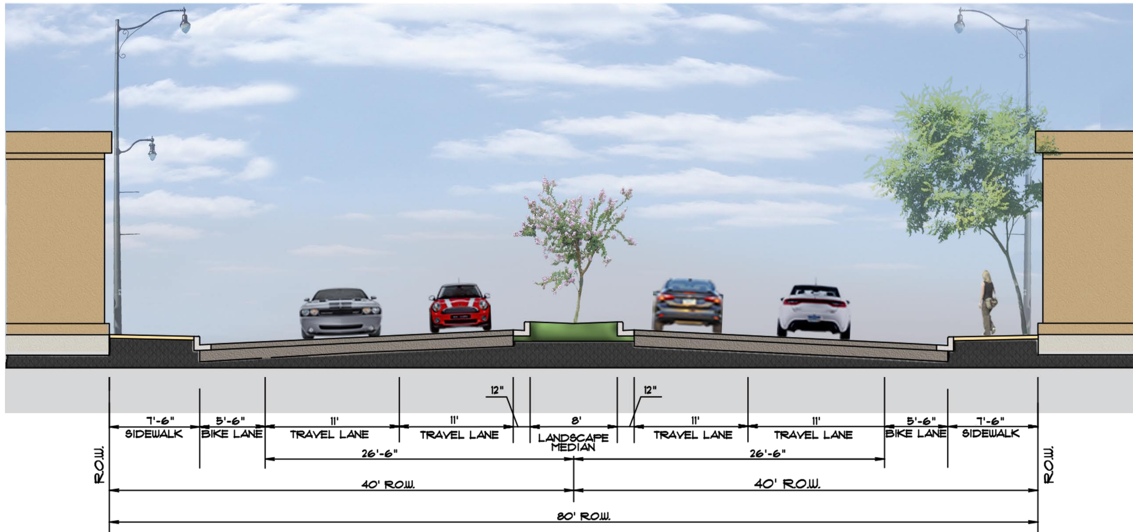
S. Federal Highway Corridor - Existing Street Section with Median
