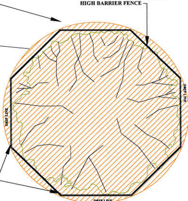
TREE PROTECTION FENCE PLAN
